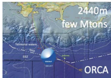
Neutrino Oscillations Mass Hierarchy
