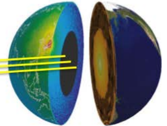
Earth: \sim 10^9 /second
