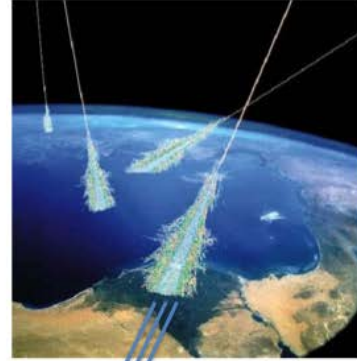
Atmosphere: \sim 20 /second
